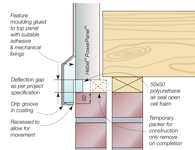
Detail 17.7.3 Horizontal Control Joint - Cavity Brickwork to Hebel™ PowerPanel™
