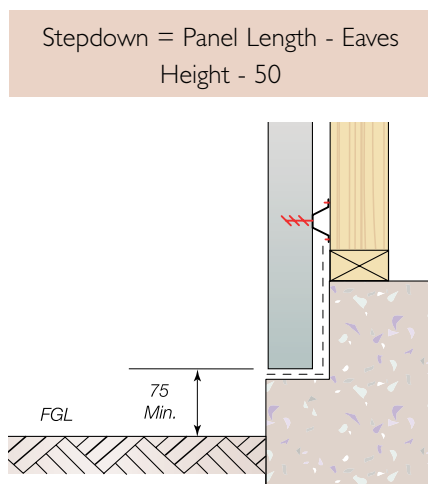
Fig. 12.1 Typical Stepdown Detail
