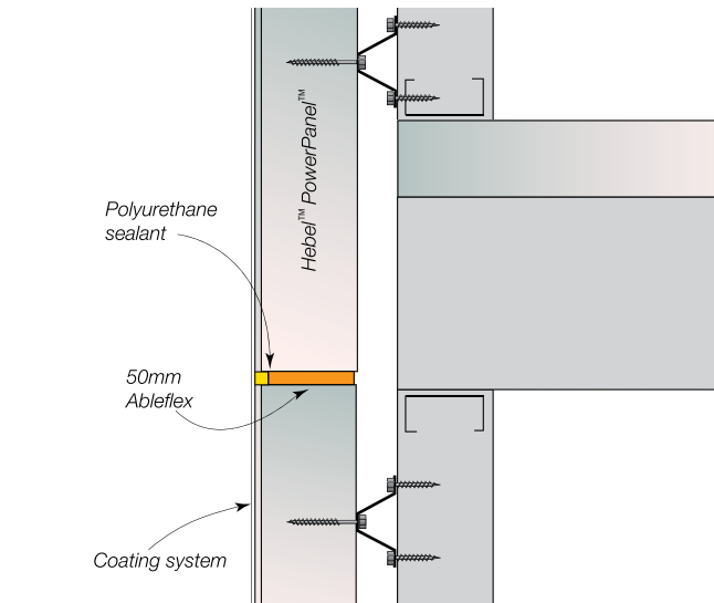
Detail 17.7.2 Typical Horizontal Control Joint - Steel Stud Frame
