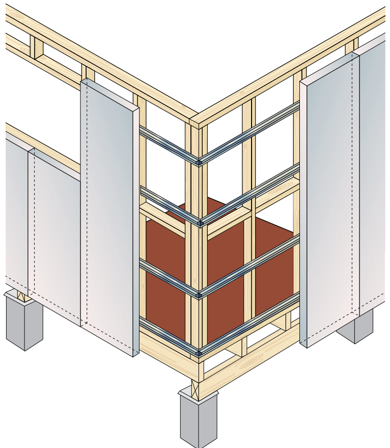
Detail 17.1.1 Single Storey Construction - Isometric View Detail Panel Suspended
