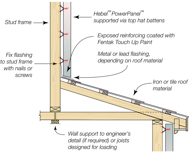
Detail 17.6.5 2nd Storey Wall Set Back Detail
