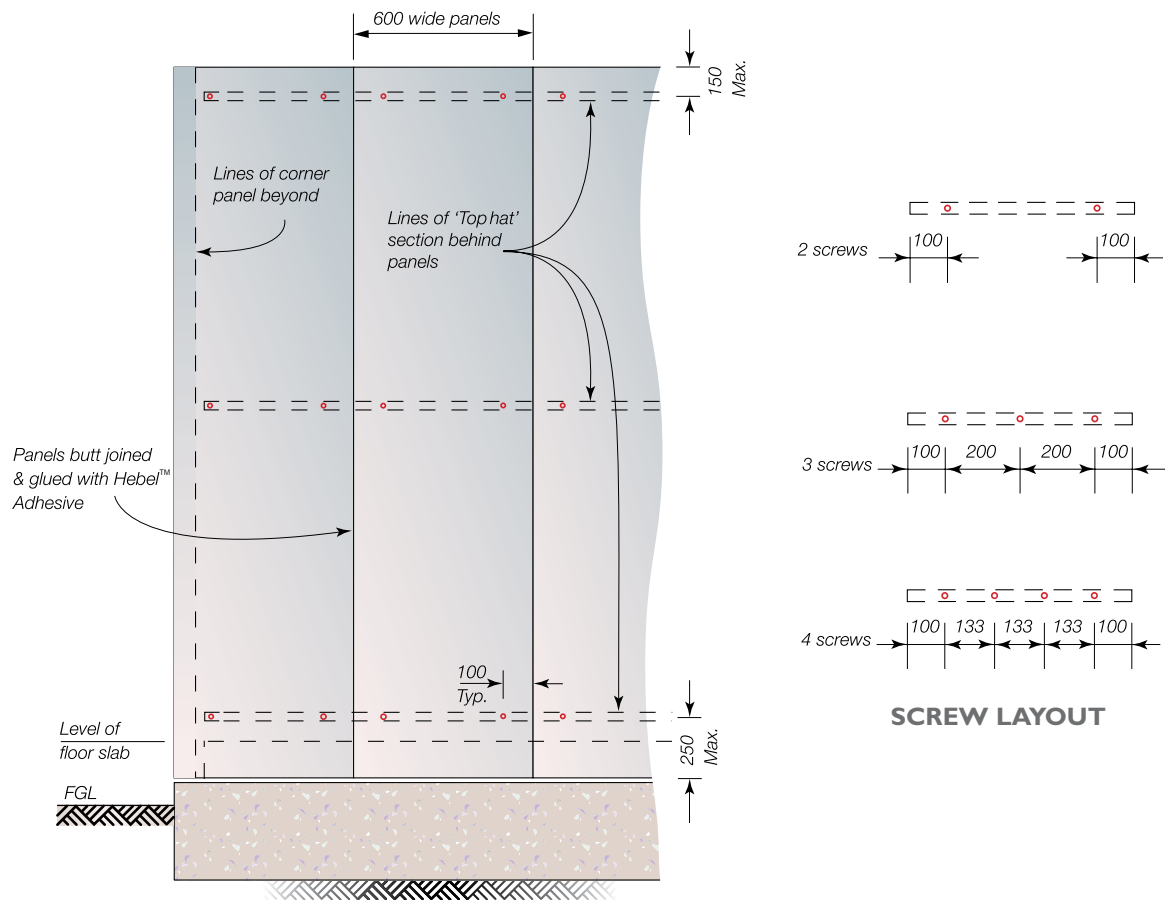
POWERPANEL™ SETOUT - ELEVATION VIEW
