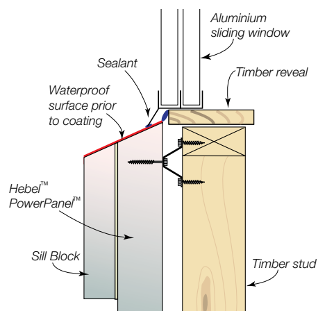
Detail 17.8.8 Sill Detail
