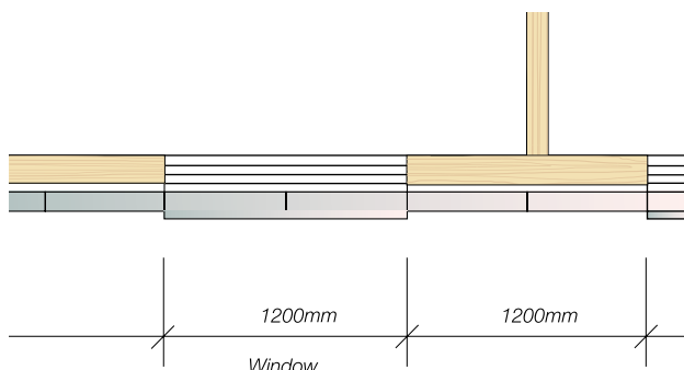
Fig. 12.4 Typical Modular Layout of Window
