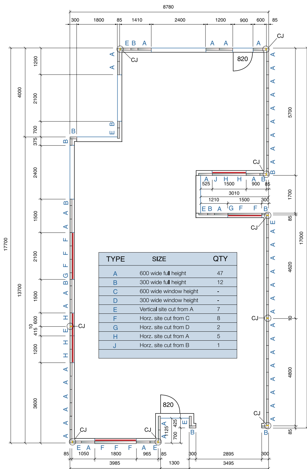
Detail 17.9.1 Panel Layout drawing - Plan View
