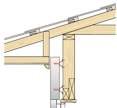
Fig. 12.3 Typical Window Head Detail
