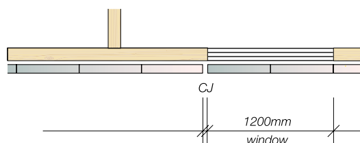
Fig. 12.6 Typical Control Joint Detail
