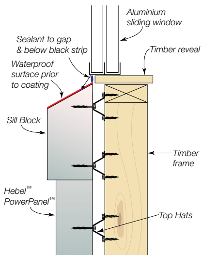
Detail 17.8.4 Typical Window Sill Detail & Timber Window Frame
