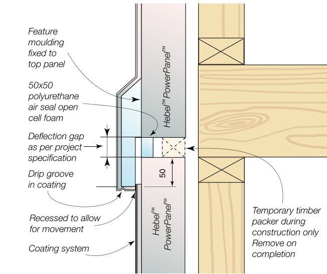
Detail 17.7.1 Typical Horizontal Control Joint - Timber Stud Frame
