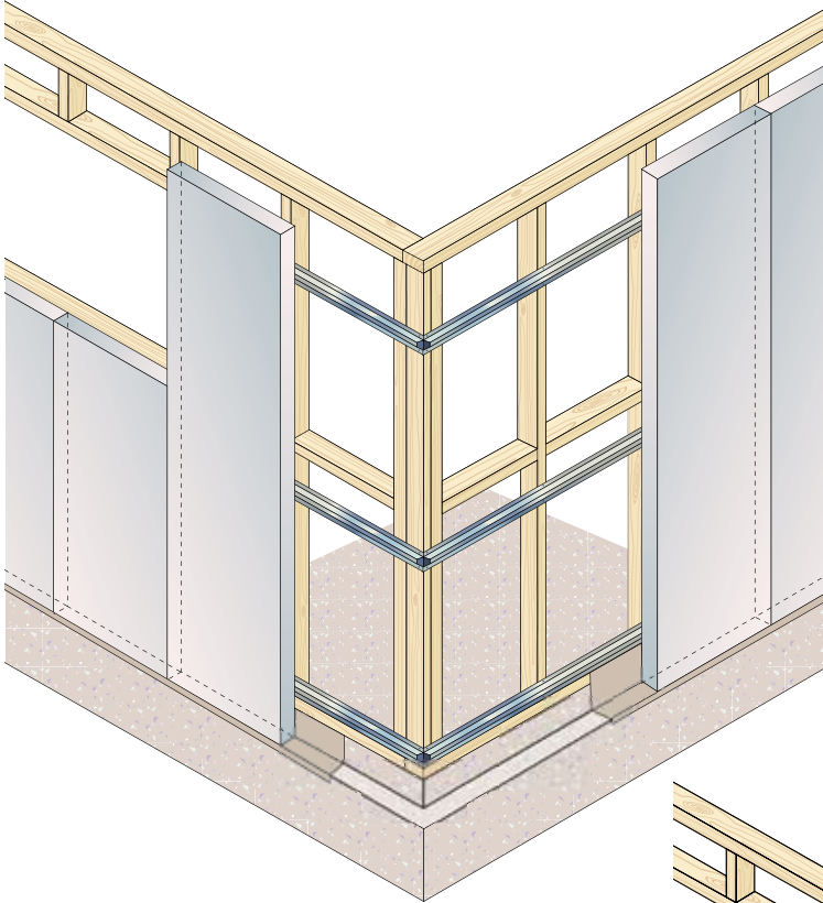
Detail 17.1.0 Single Storey Construction - Isometric View Detail Panel Supported at Base
