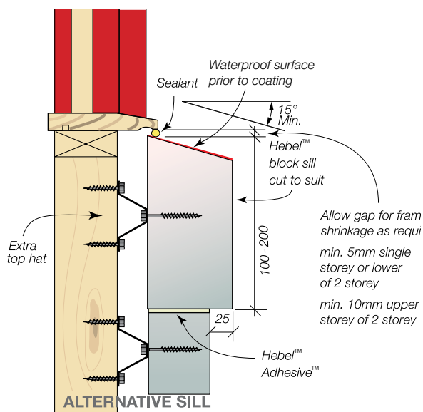
Detail 17.8.5 Alternative Window Sill Detail - Timber Frame Window
