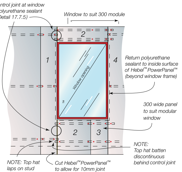
Detail 17.8.2 Typical Window Control Joint Detail - Lintel Over
