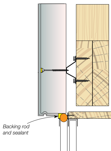
Detail 17.8.6 Header Detail
