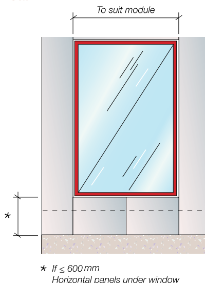
Fig.12.8 Panels Below Window Detail
