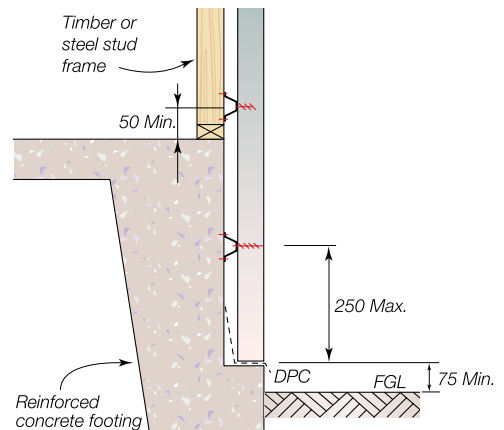
Detail 17.5.2 Footing Junction Detail 2
