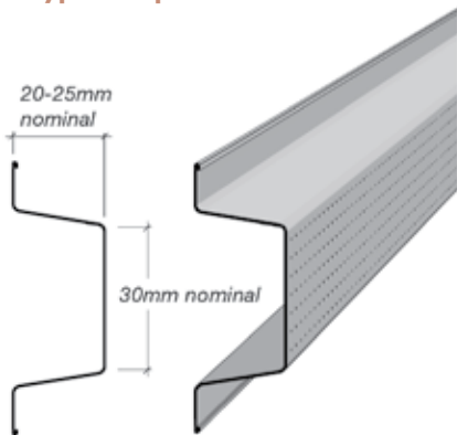
Fig. 13.1 Typical tophat
