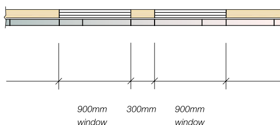
Fig.12.10 Typical Panel Layout for Window
