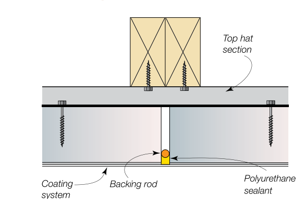
Detail 17.7.6 Typical Dummy Joint
