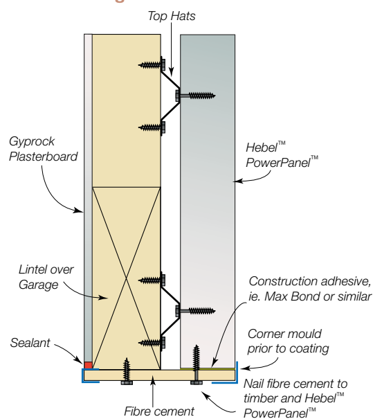
Detail 17.8.9 Garage Head Detail
