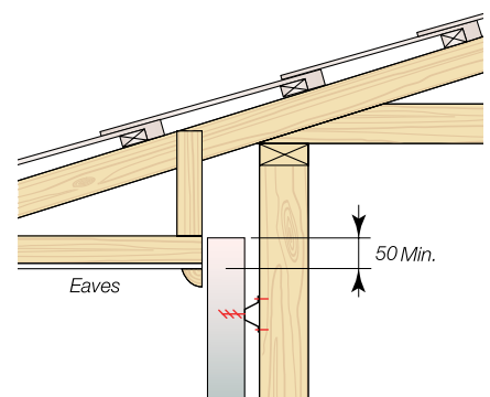
Fig. 12.2 Typical Eaves Detail
