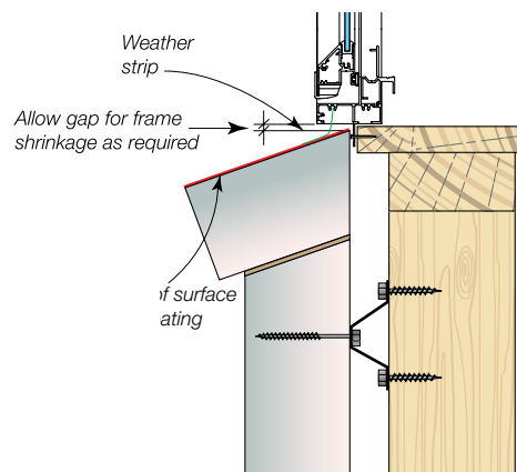
Detail 17.8.9 Garage Head Detail
